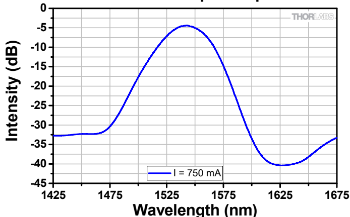
SLD1550P-A40 Optical Spectrum
