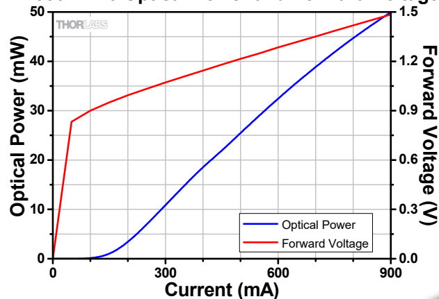
SLD1550P-A40 Optical Power and Forward Voltage
