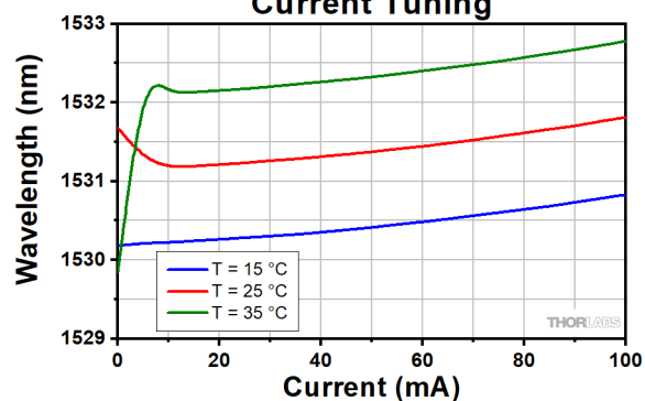
DFB1531 Temperature and Current Tuning
