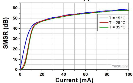
DFB1531 Side Mode Suppression Ratio
