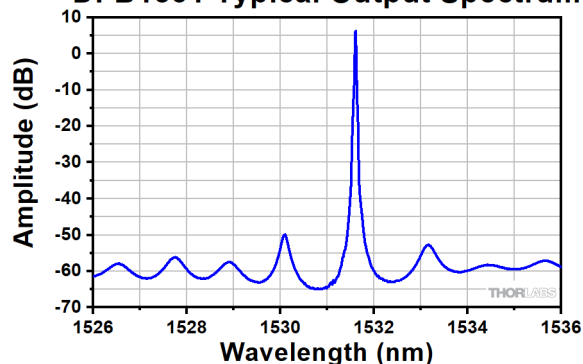
DFB1531 Typical Output Spectrum
