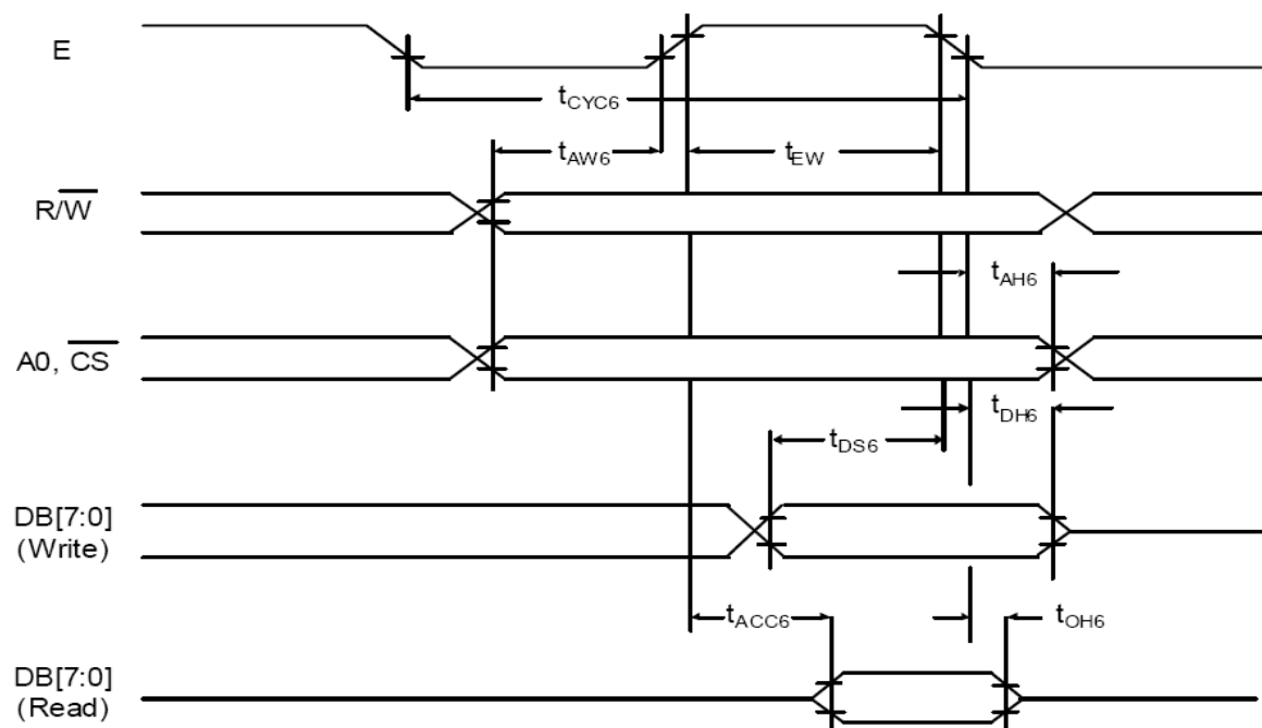
Figure 1: 6800 MCU Waveform
