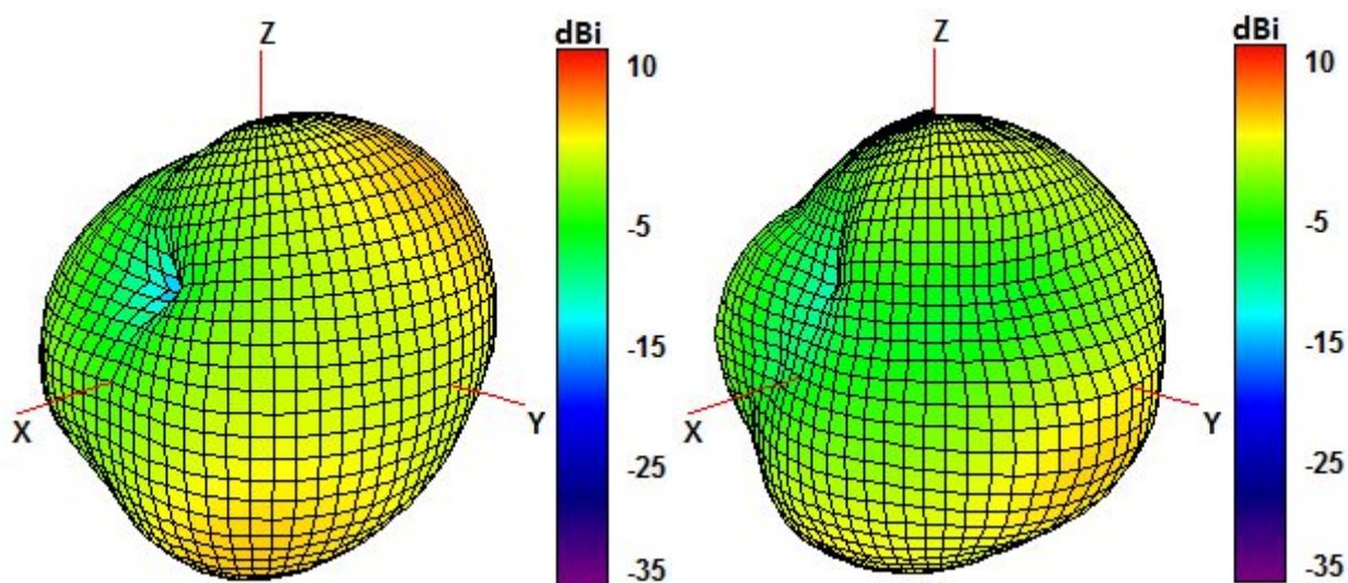
Cable 2: CELLULAR/LTE
