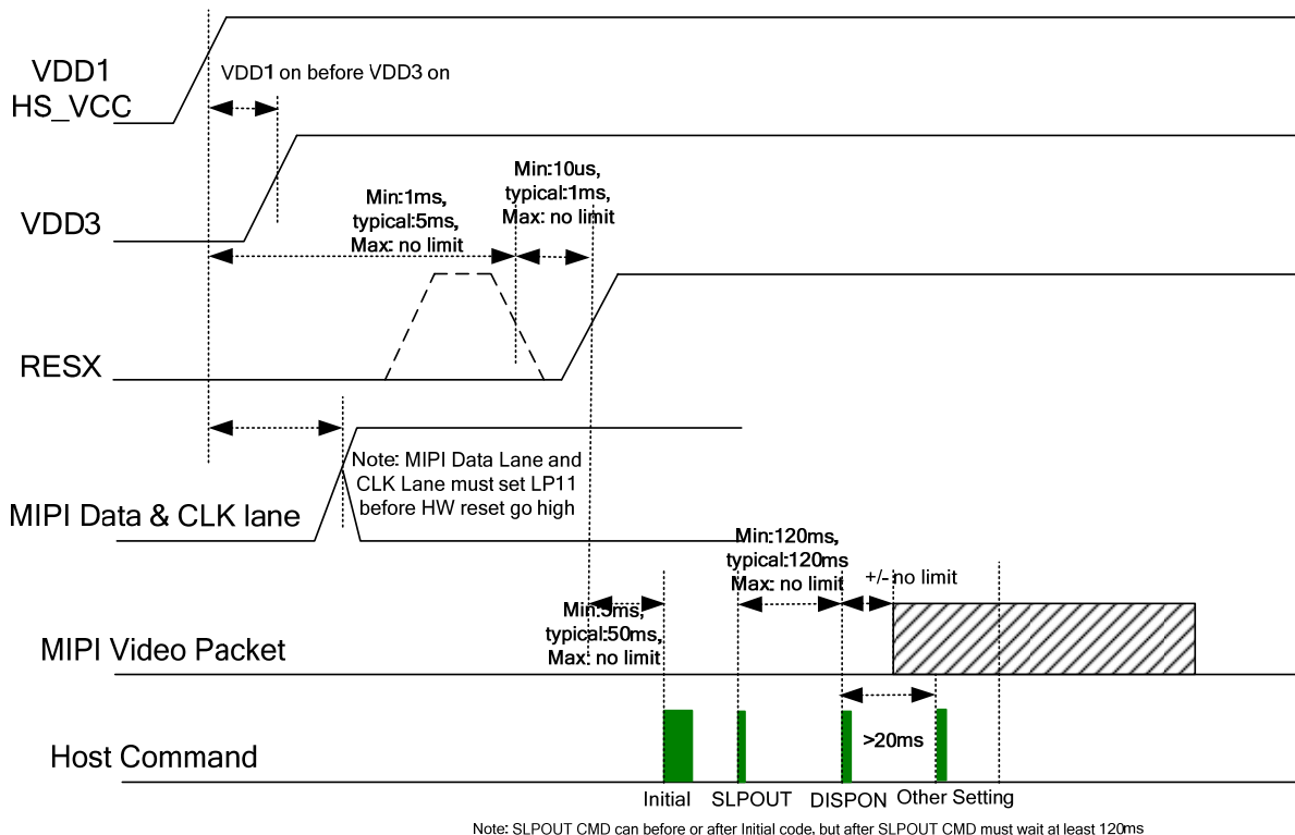
Figure 5.28: VDD1/VDD3 input power on sequence
