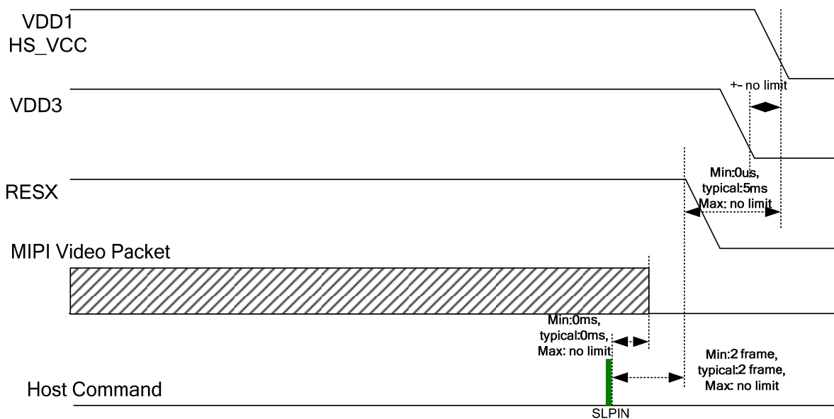
Figure 5.29: VDD1/VDD3 input power off sequence
