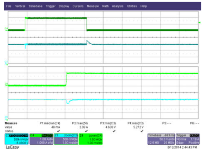
Figure 25 – Transient Response ( 4.6 V_{\text{MIN}} ). 265 VAC, 0-2 A Load Step. Upper: I_{\text{LOAD}} , 1 A / div. Lower: V_{\text{OUT}} , 500 mV, 50 ms / div.
