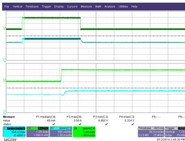
Figure 29 – Transient Response ( 4.86 V_{MIN} ). 265 VAC, 0-2 A Load Step. Upper: I_{LOAD} , 1 A / div. Lower: V_{OUT} , 500 mV, 50 ms / div.
