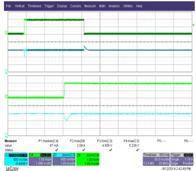
Figure 23 – Transient Response ( 4.5 V_{\text{MIN}} ). 110 VAC, 0-2 A Load Step. Upper: I_{\text{LOAD}} , 1 A / div. Lower: V_{\text{OUT}} , 500 mV, 50 ms / div.
