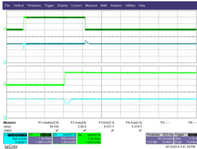
Figure 22 – Transient Response ( 4.5 V_{\text{MIN}} ). 85 VAC, 0-2 A Load Step. Upper: I_{\text{LOAD}} , 1 A / div. Lower: V_{\text{OUT}} , 500 mV, 50 ms / div.
