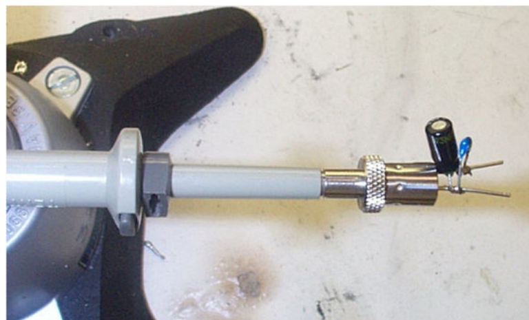
Figure 35 – Oscilloscope Probe with Probe Master ( www.probemaster.com ) 4987A BNC Adapter. (Modified with wires for ripple measurement, and two parallel decoupling capacitors added)
