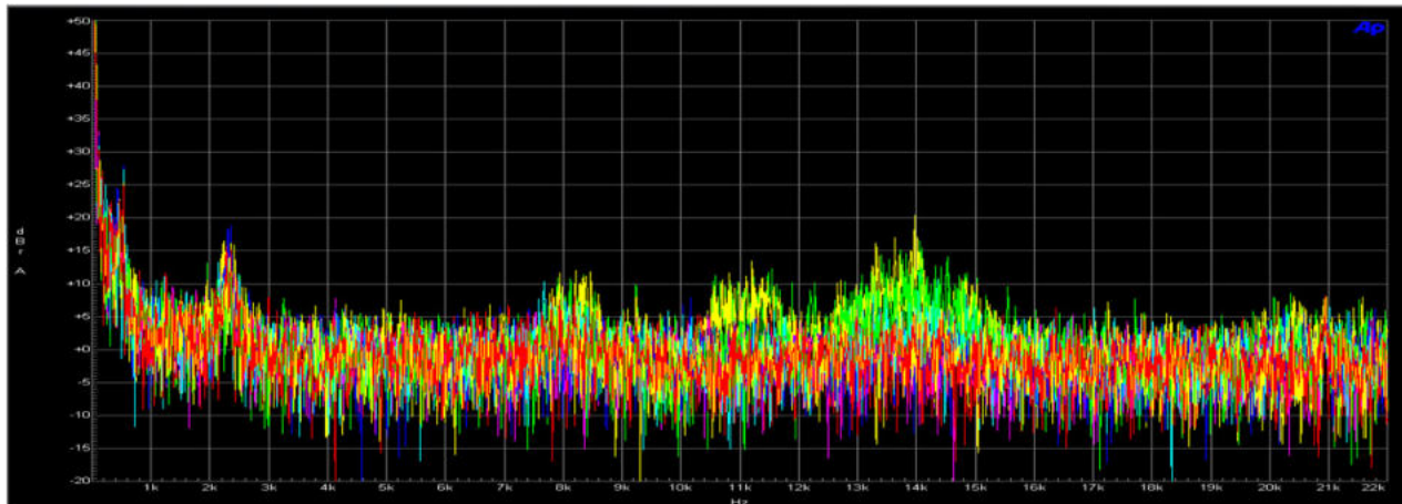
Figure 49 – Audible Noise Spectrum: 265 VAC, I_{OUT} Swept from 0 A to 2.0 A.
