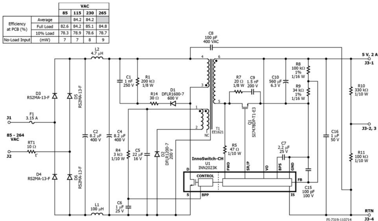
Figure 3 – Schematic.
