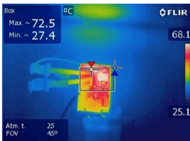
Figure 19 – InnoSwitch-CH Side. 230 VAC, 2 A Load. Ambient = 25.4 °C.
