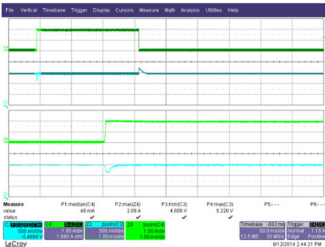
Figure 24 – Transient Response ( 4.6 V_{\text{MIN}} ). 230 VAC, 0-2 A Load Step. Upper: I_{\text{LOAD}} , 1 A / div. Lower: V_{\text{OUT}} , 500 mV, 50 ms / div.
