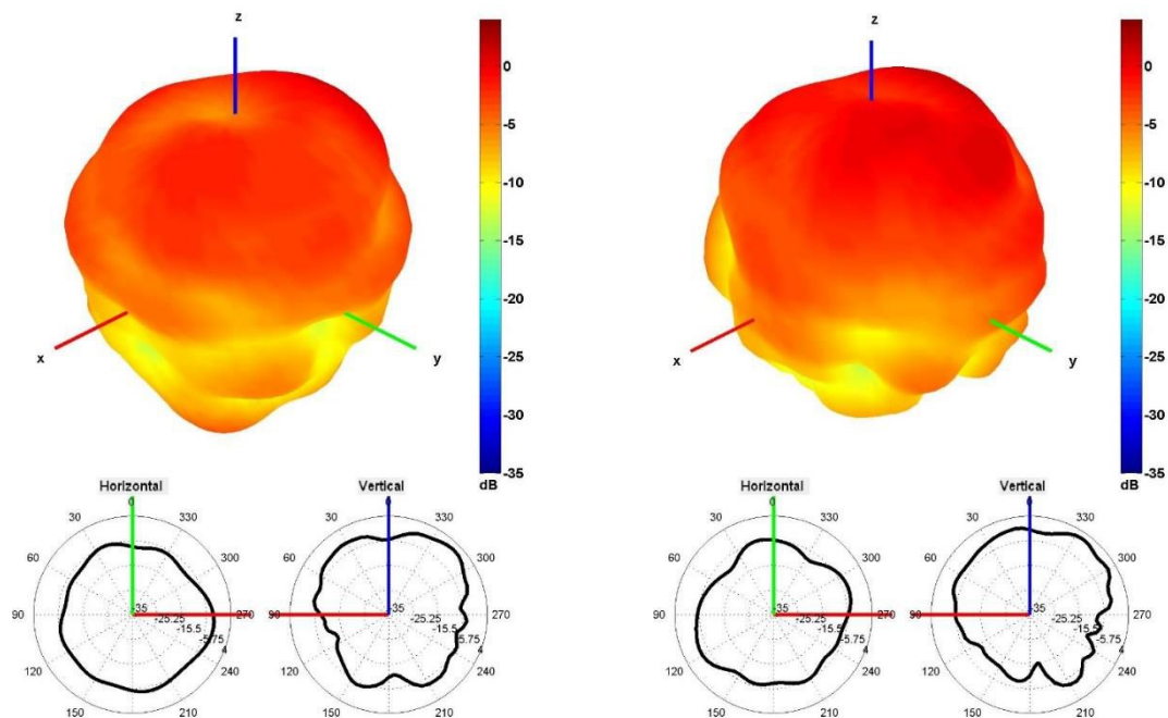
850 and 940 MHz Radiation pattern
