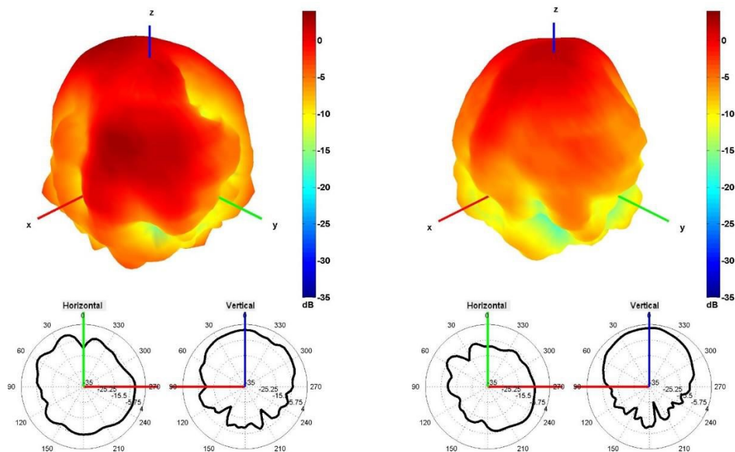
1950 and 2100 MHz Radiation pattern
