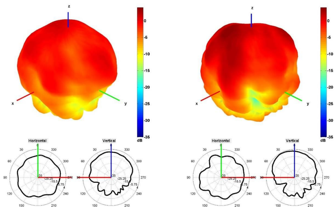
1750 and 1850 MHz Radiation pattern
