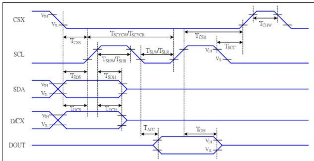
Figure7.1.1 4-line serial Interface Timing Characteristics
