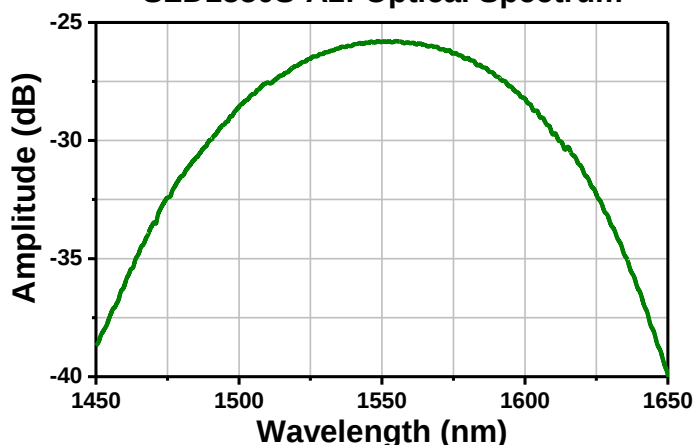
SLD1550S-A1: Optical Spectrum
