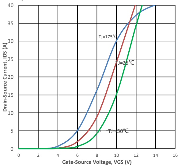
Fig5. Transfer Characteristic
