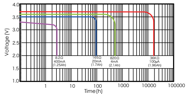
1. Typical discharge profiles at 23±2°C (at the mid-discharge)
