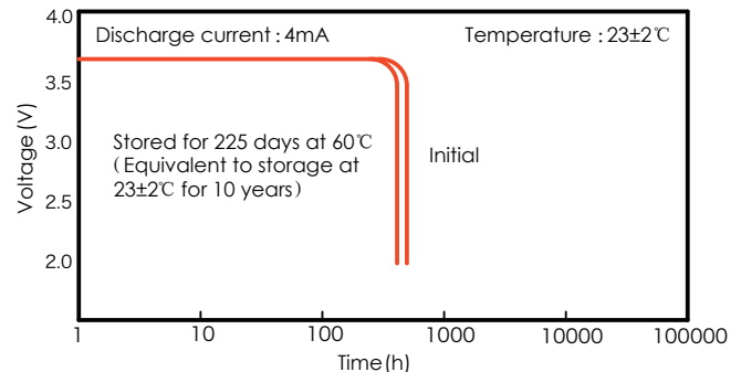
3. Storage characteristics
