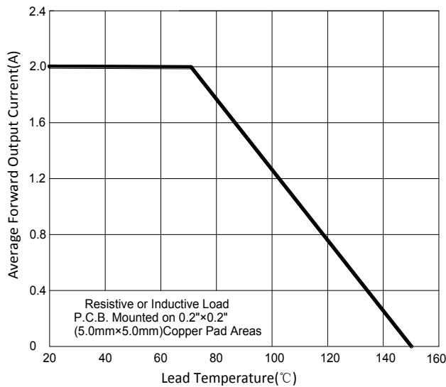
FIG1: Io-TL Curve
