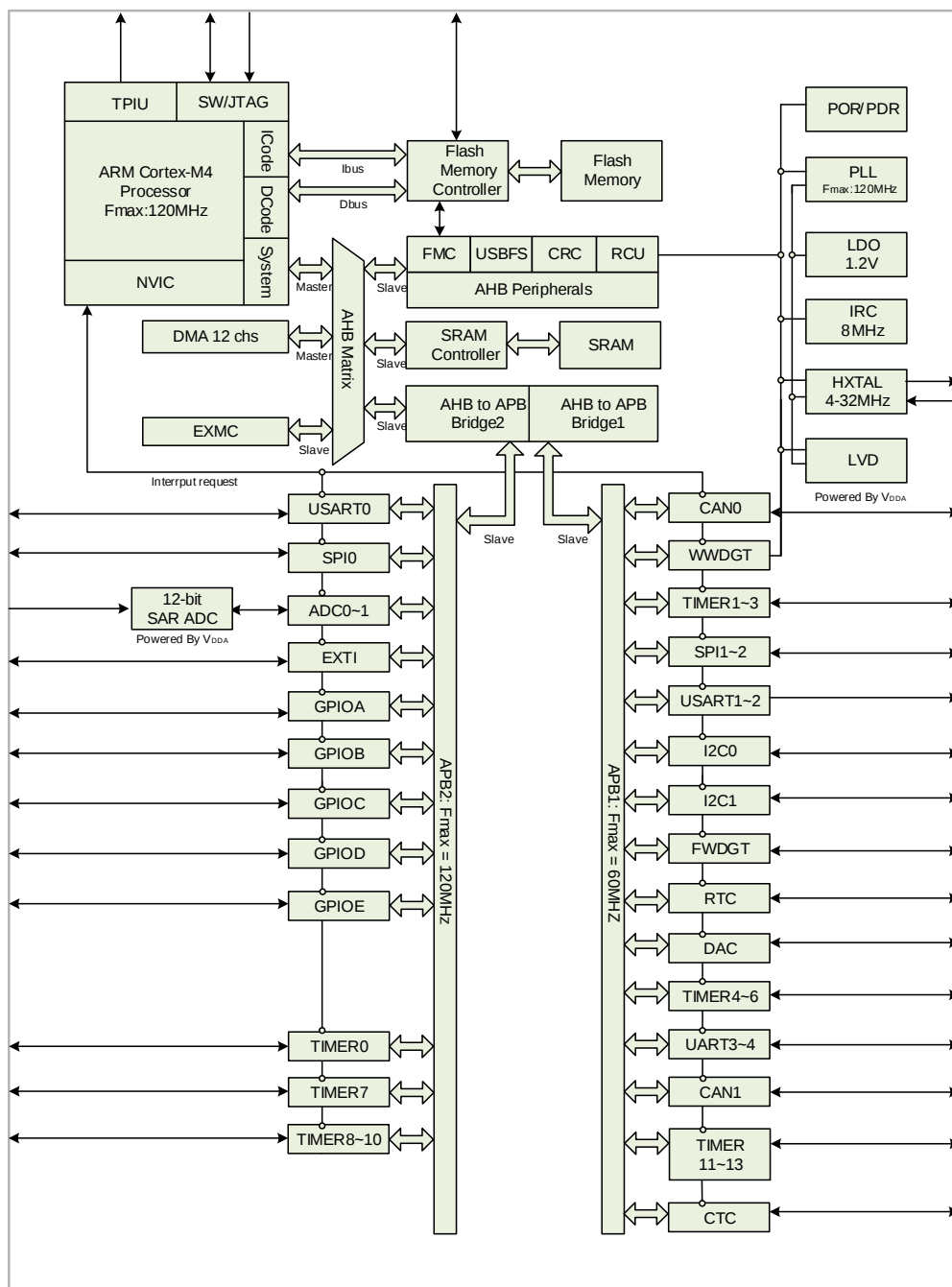
Figure 2-1.GD32C113xx block diagram
