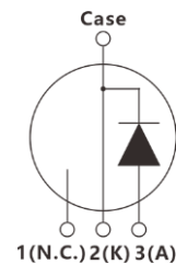
Inner Circuit
