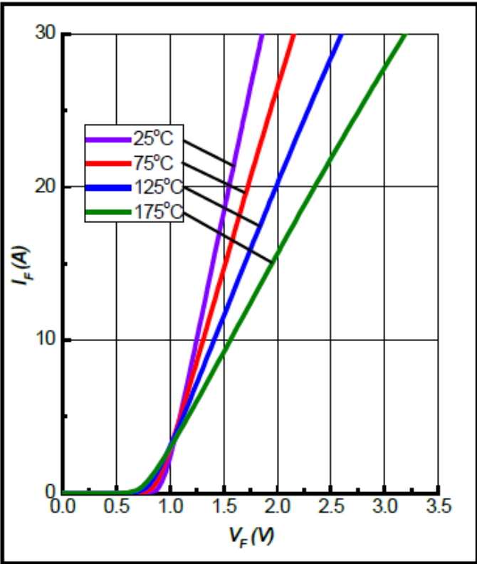
Figure 1. Forward Characteristics
