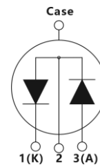
Inner Circuit
