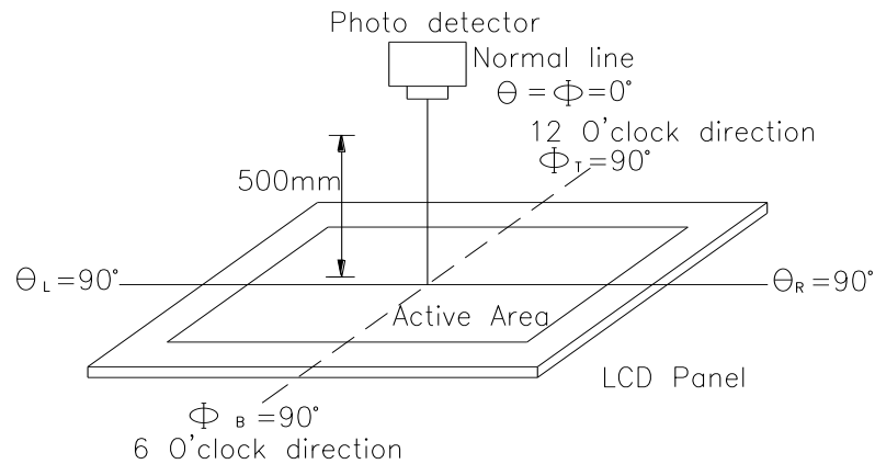
Fig. 12.2. Optical measurement system setup
