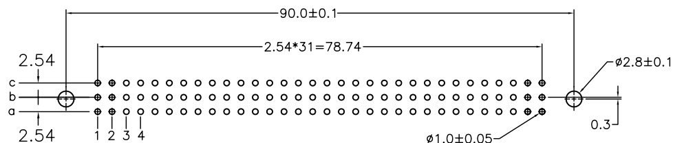
P.C. Board Layout
