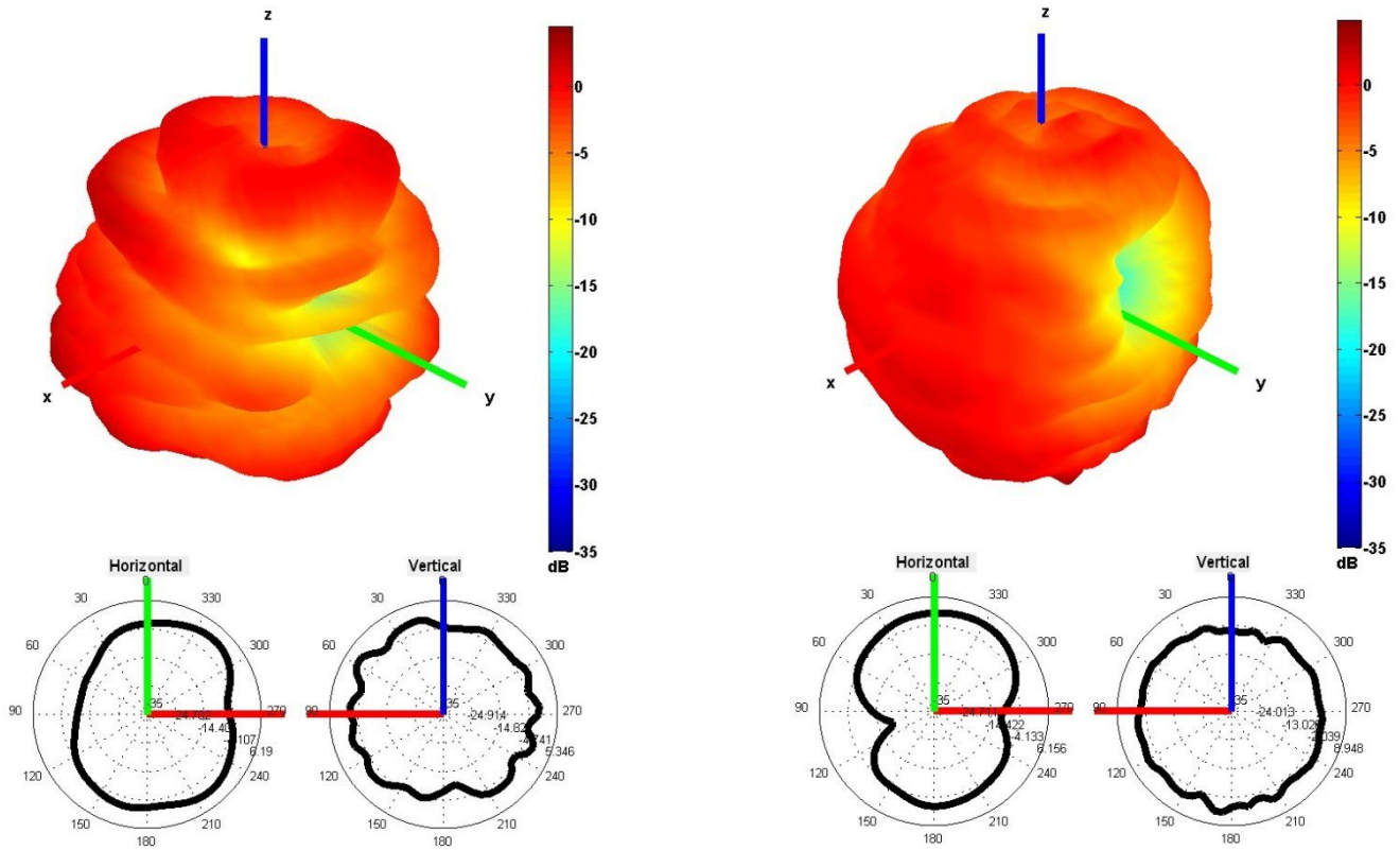
940 and 1750 MHz Radiation pattern
