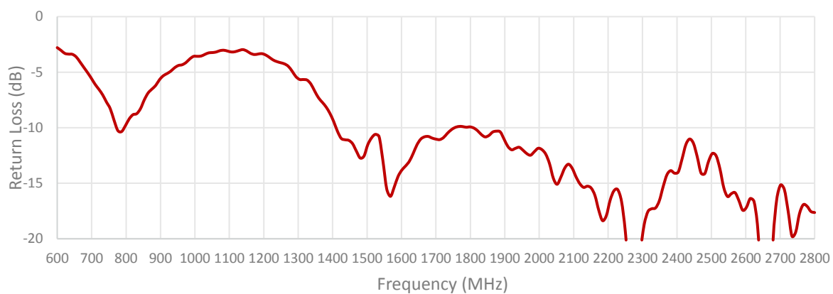
Cable 1: CELLULAR/LTE
