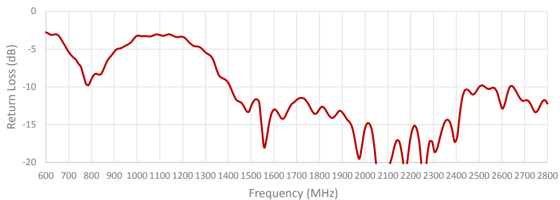
Cable 2: CELLULAR/LTE
