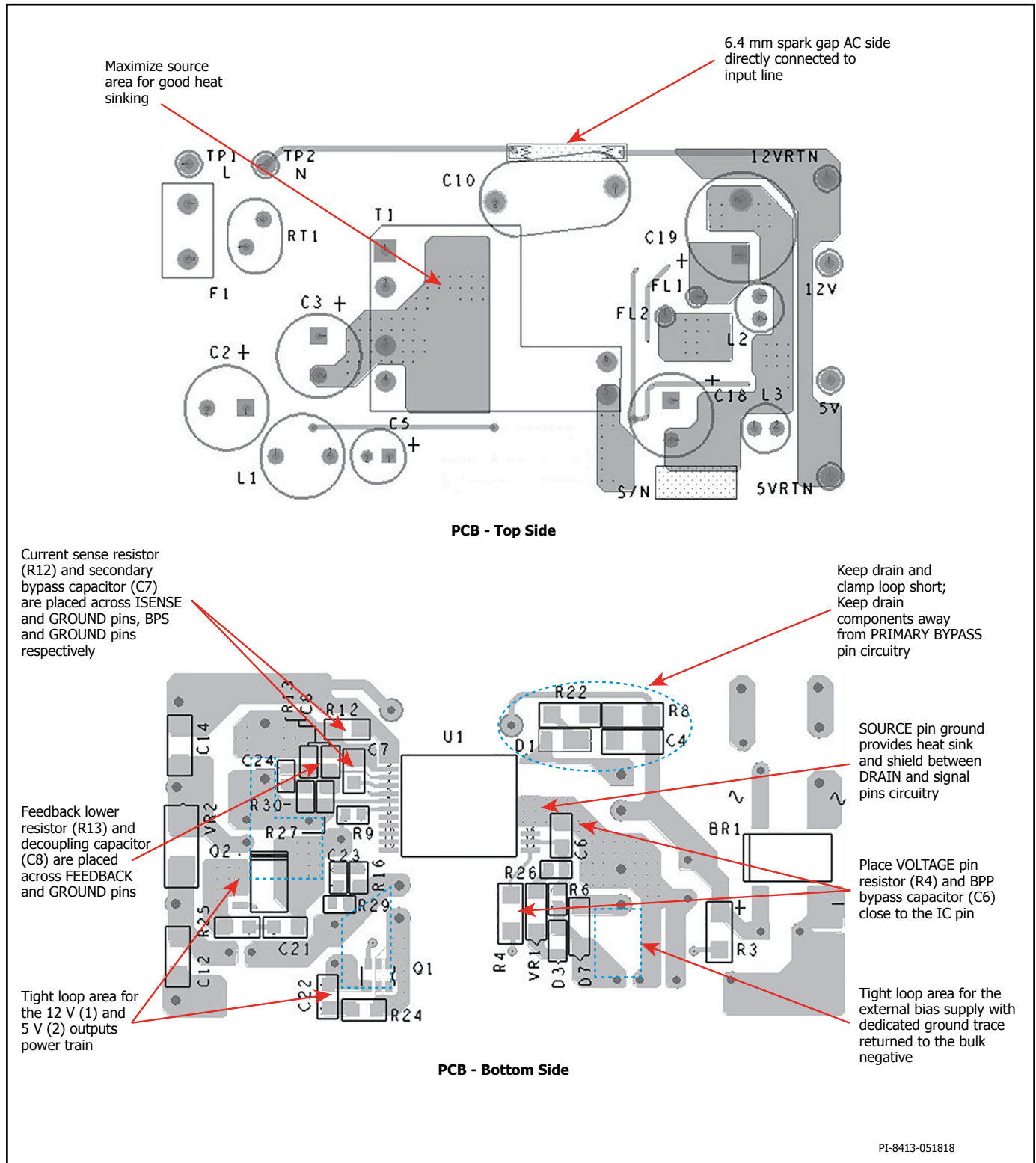
Figure 17. PCB.
