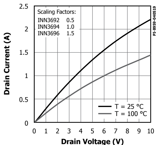
Figure 27. Output Characteristics.
