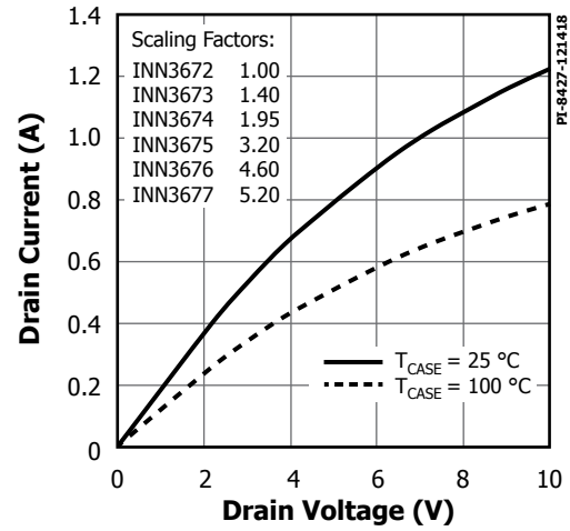
Figure 21. Output Characteristics.
