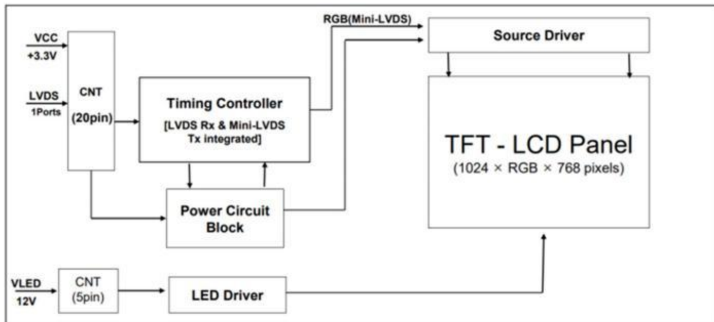
Figure 1. Drive Architecture
