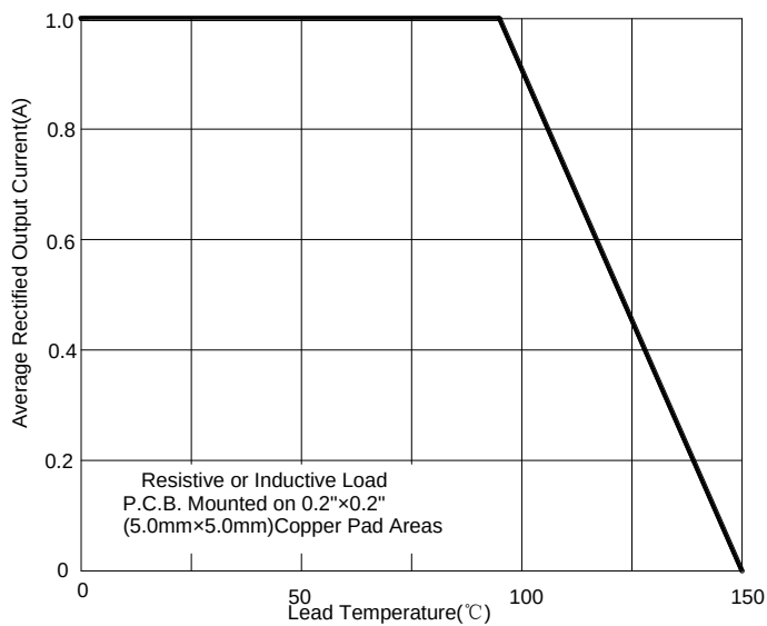
FIG.1: IO-TL Curve
