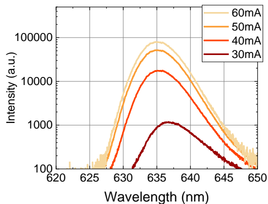
typical spectra
