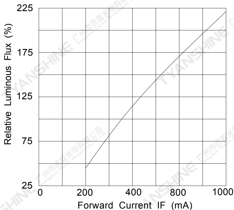
Forward Current VS. Relative Luminous Flux
