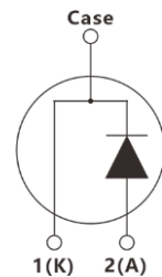
Inner Circuit
