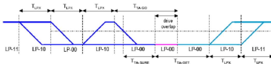
Figure 4.4 : Turnaround Procedure
