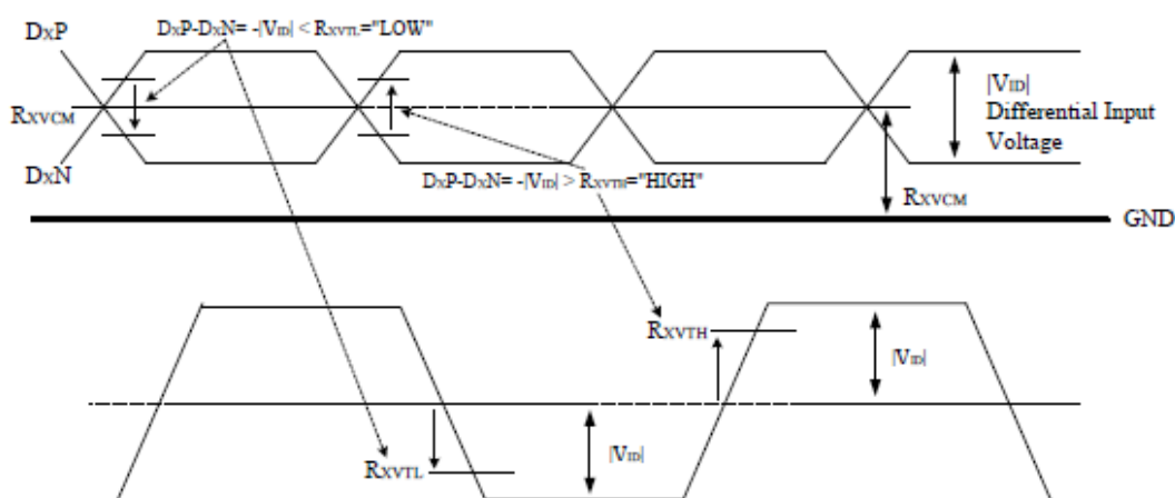
Single-end Signals
