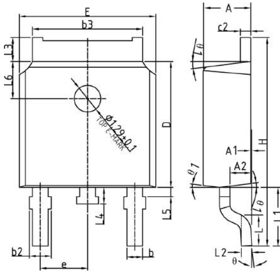
TO-252 DPAK
