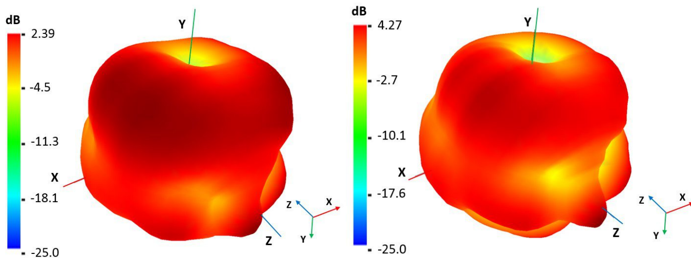
1750 and 1850 MHz Radiation pattern
