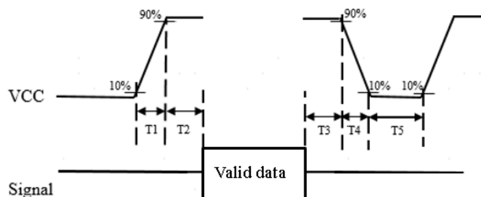
Power on/off signal sequence
