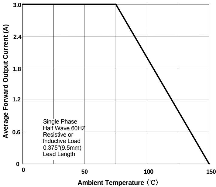
FIG.1: Io-Ta Curve
