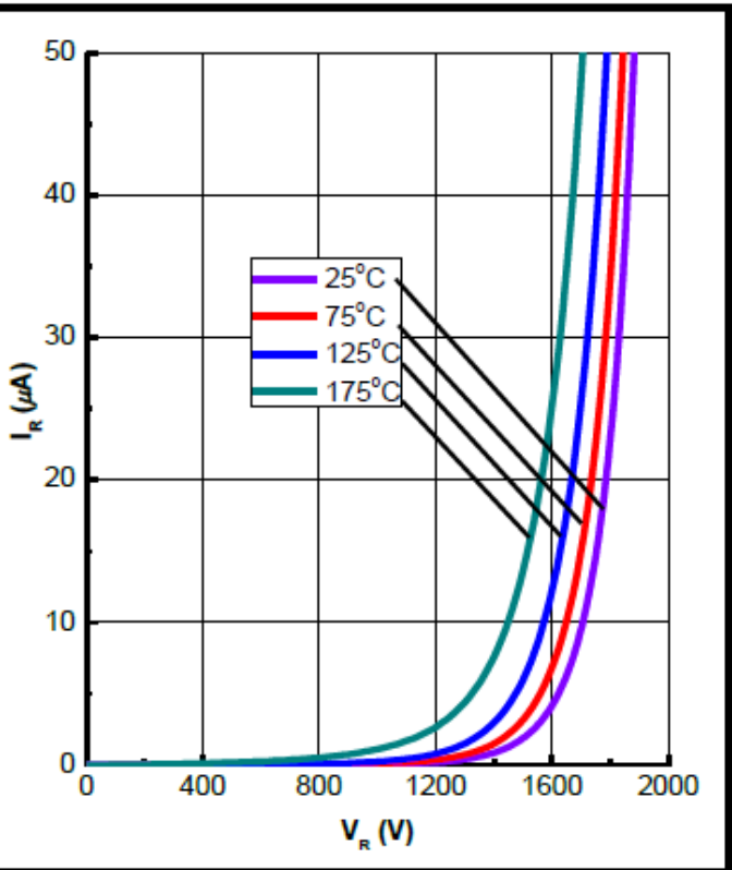
Figure 2. Reverse Characteristics
