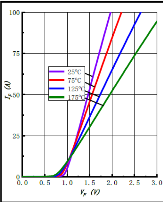
Figure 1. Forward Characteristics
