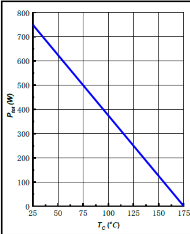
Figure 3. Power Derating
