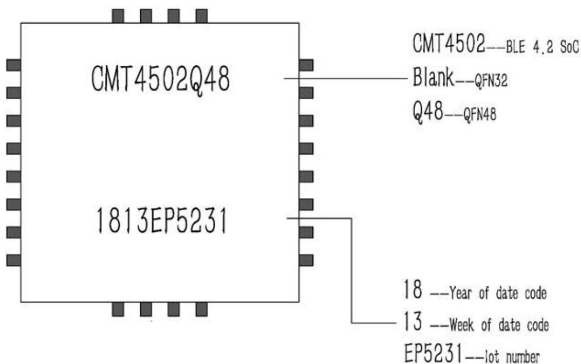
Figure 14: Chip Marking
