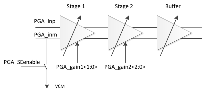
Figure 13: PGA path
