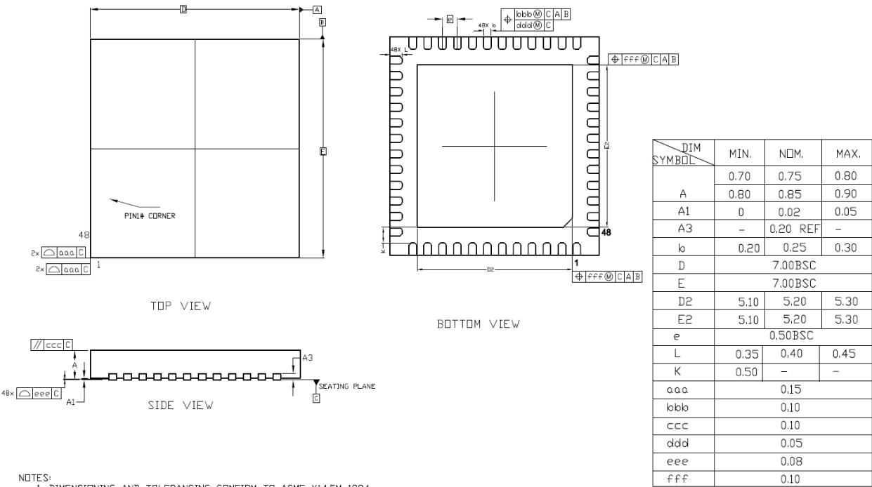
Figure 16: QFN48 package dimensions
